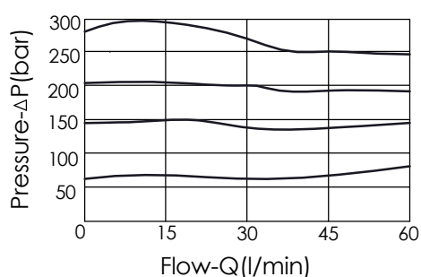
Typical Relief Characteristics
