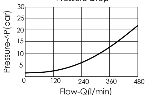
Free Flow or Piloted Open Pressure Drop
