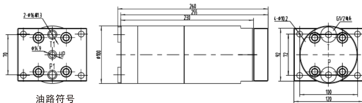
Dimensions of Flange Mounting
